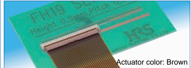
FH19SC – FPC/FFC thickness: 0.3±0.03mm
