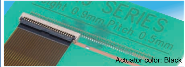
FH19SC – FPC/FFC thickness: 0.3±0.03mm
