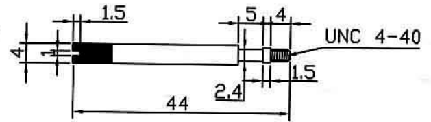
LONG SCREWS WITH SLOTTED x 2 PCS
