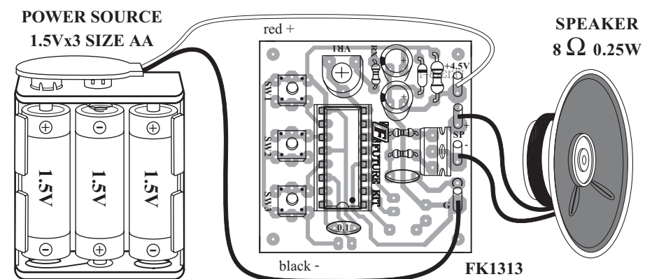
Figure 2. Circuit Assembling
