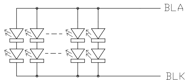
Backlight Circuit No. of LED=41x2 Scale=free
