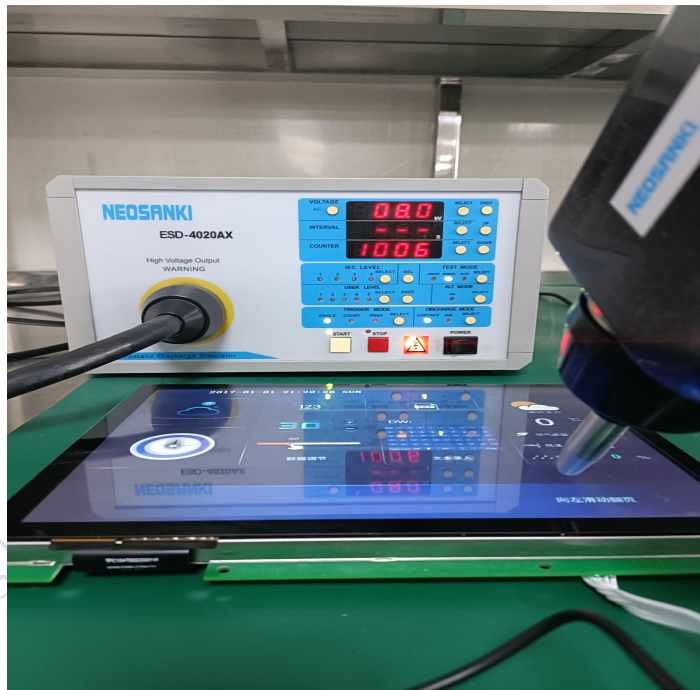
Electrostatic discharge test
