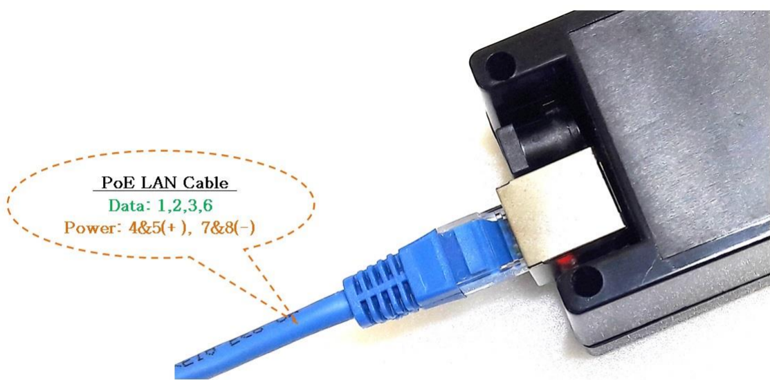
RJ-45형 PD(Powered Device) 결선
