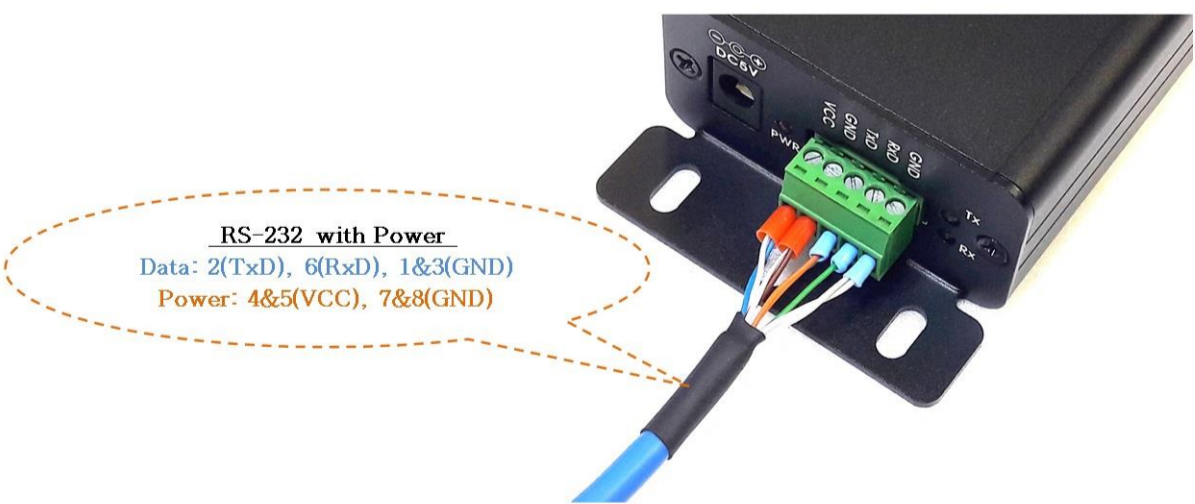
RS-232 with Power Pinmap
