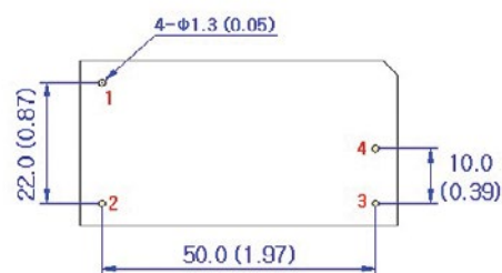
Mounting Hole (Top View)
