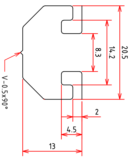
SCALE 2:1 DETAIL 'T'홀
