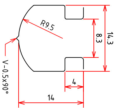
SCALE 2:1 DETAIL 'T'홀
