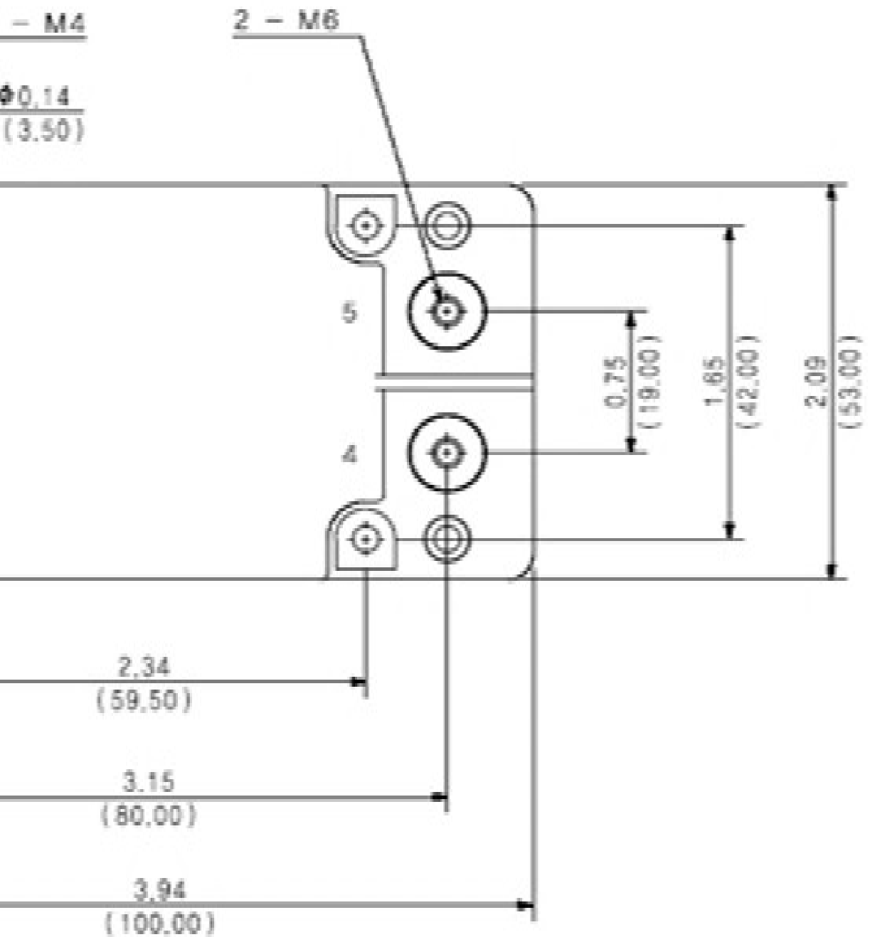
TOP VIEW
