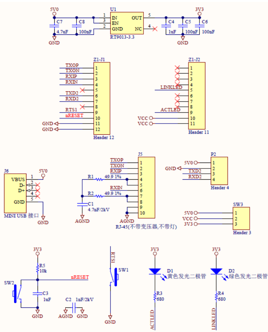
Figure 2-4 W7500S2E-R1 evaluation board reference schematic
