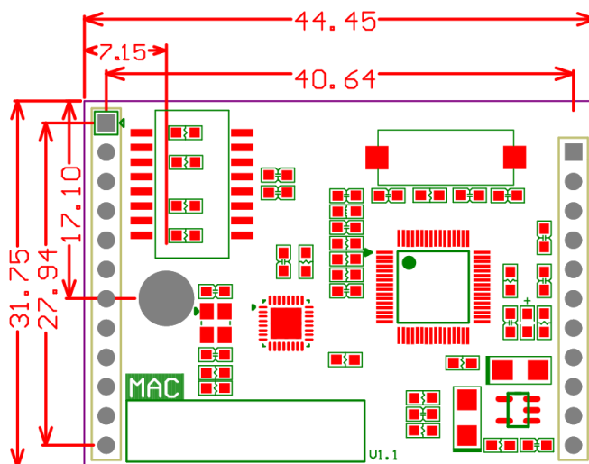
Figure 1-1 W7500S2E-R1 dimensions top view
