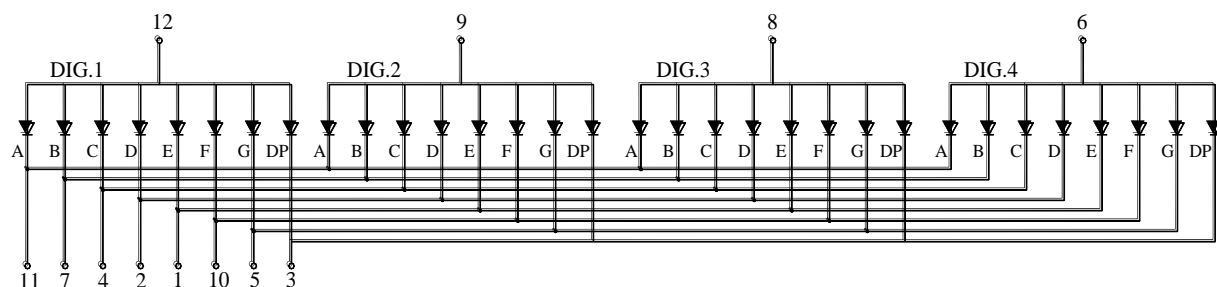
YDUR-40561AM (Common Anode)
