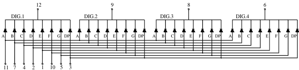
YDSR-40561KM (Common Cathode)
