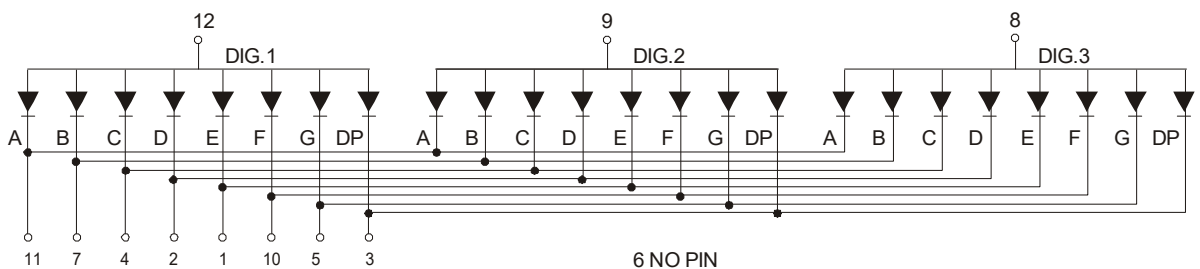
YDUG-3036AM (Common Anode)
