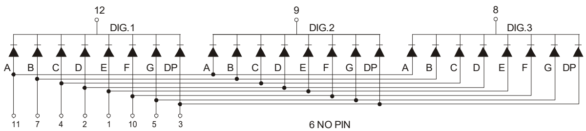
YDUG-3036KM (Common Cathode)
