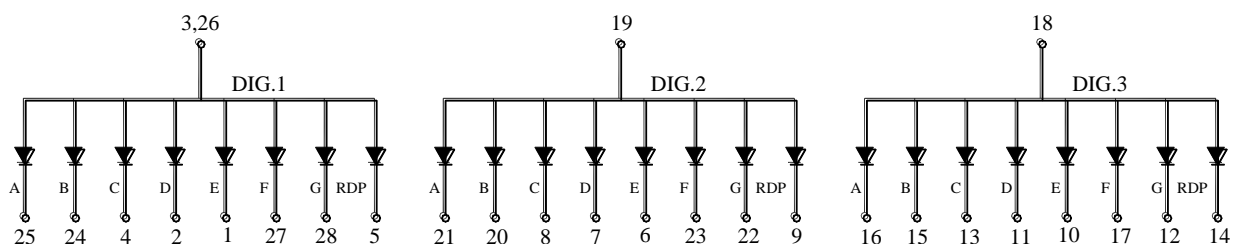
YDSR-3056AM (Common Anode)
