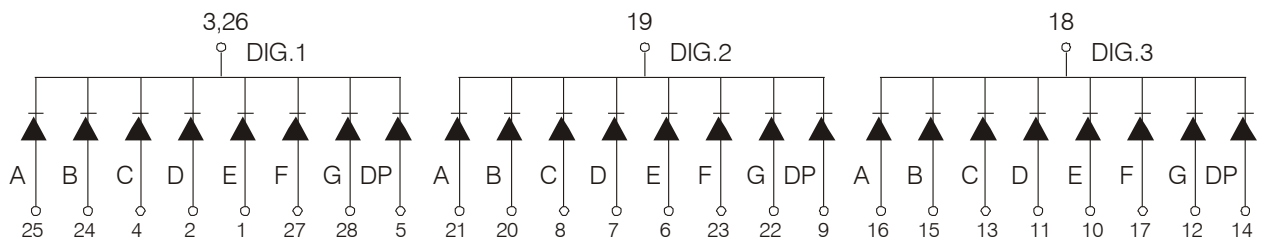
YDSR-3056KM (Common Cathode)
