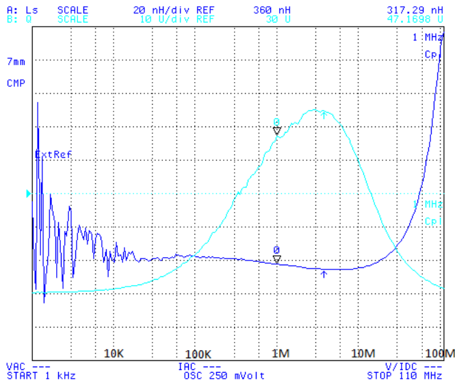
PIC252012-R68
