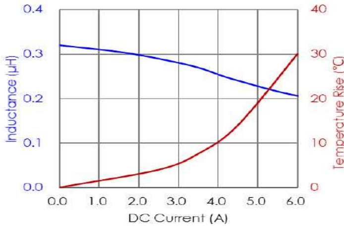
PIC252012-R33
