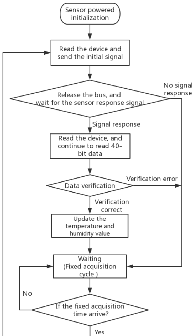
Figure 9 The Single Bus Read Flow Chart
