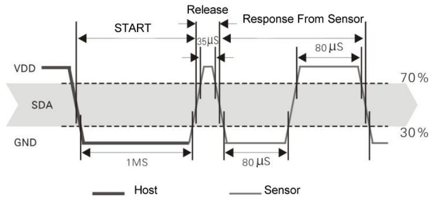
Figure 7 Single Bus Decomposition Timing Diagram
