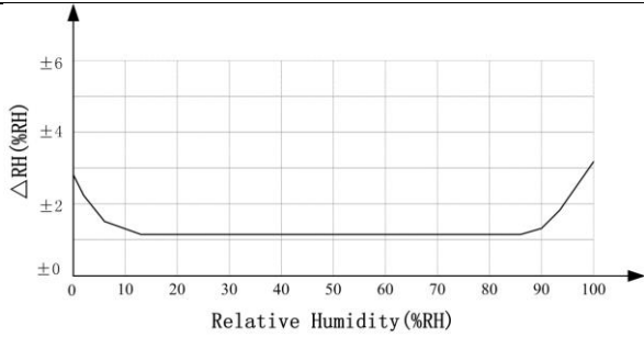
Figure 2 Typical RH% Accuracy at 25°C
