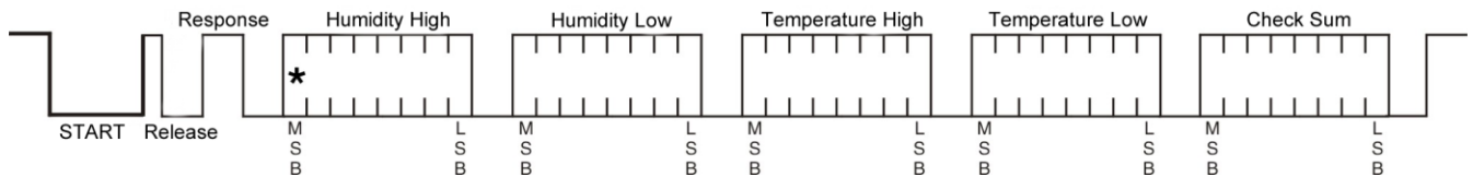
Figure 5 CM2305 Single Bus Communication Protocol
