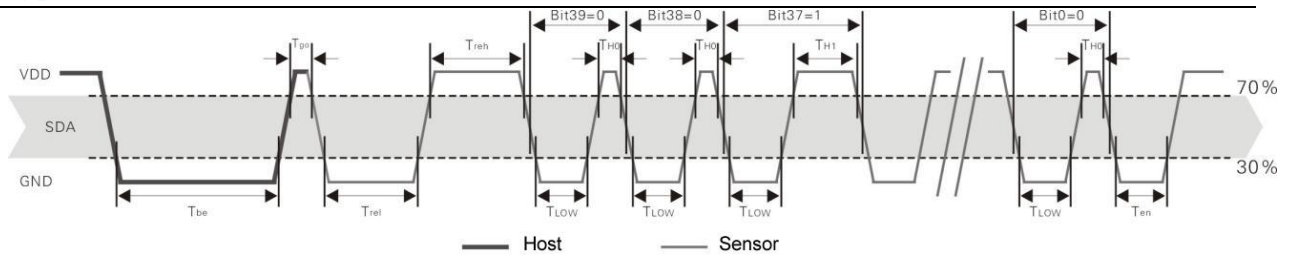
Figure 6 CM2305 Single bus communication timing
