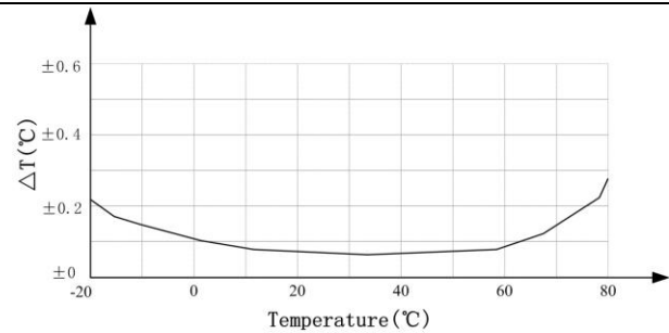
Figure 3 Typical Temperature Accuracy
