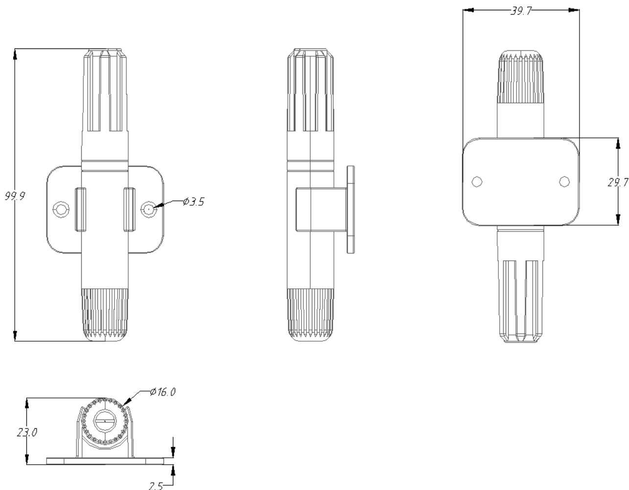
Figure 1 Dimension (Units: mm)
