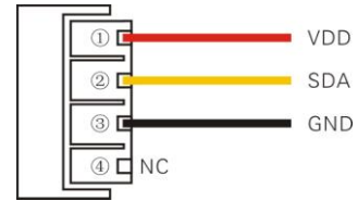
Figure 4 CM2305 Wiring Diagram
