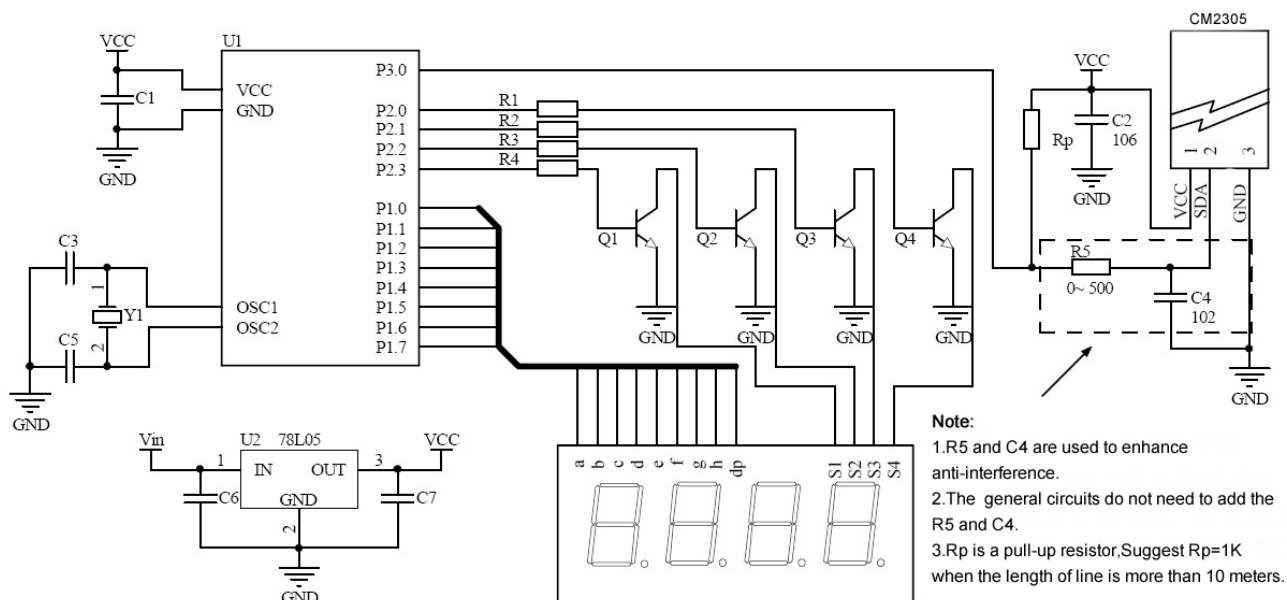
Figure 4 CM2305 One-Wire Application Circuitry
