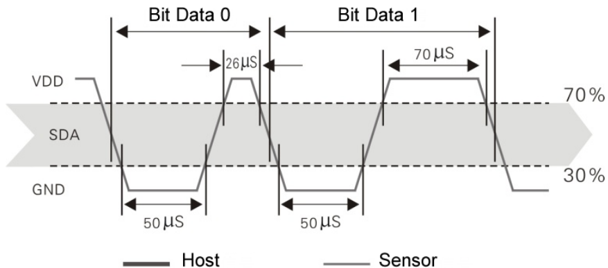
Figure 8 Single Bus Decomposition Sequence Diagram
