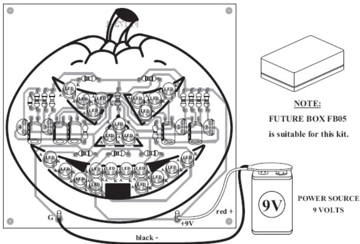
Figure 3. Connections
