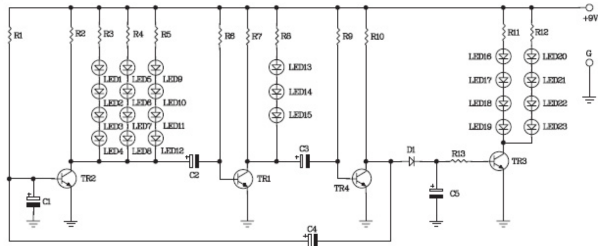
Figure 2. The halloween pumpkin flasher 23 LED circuit
