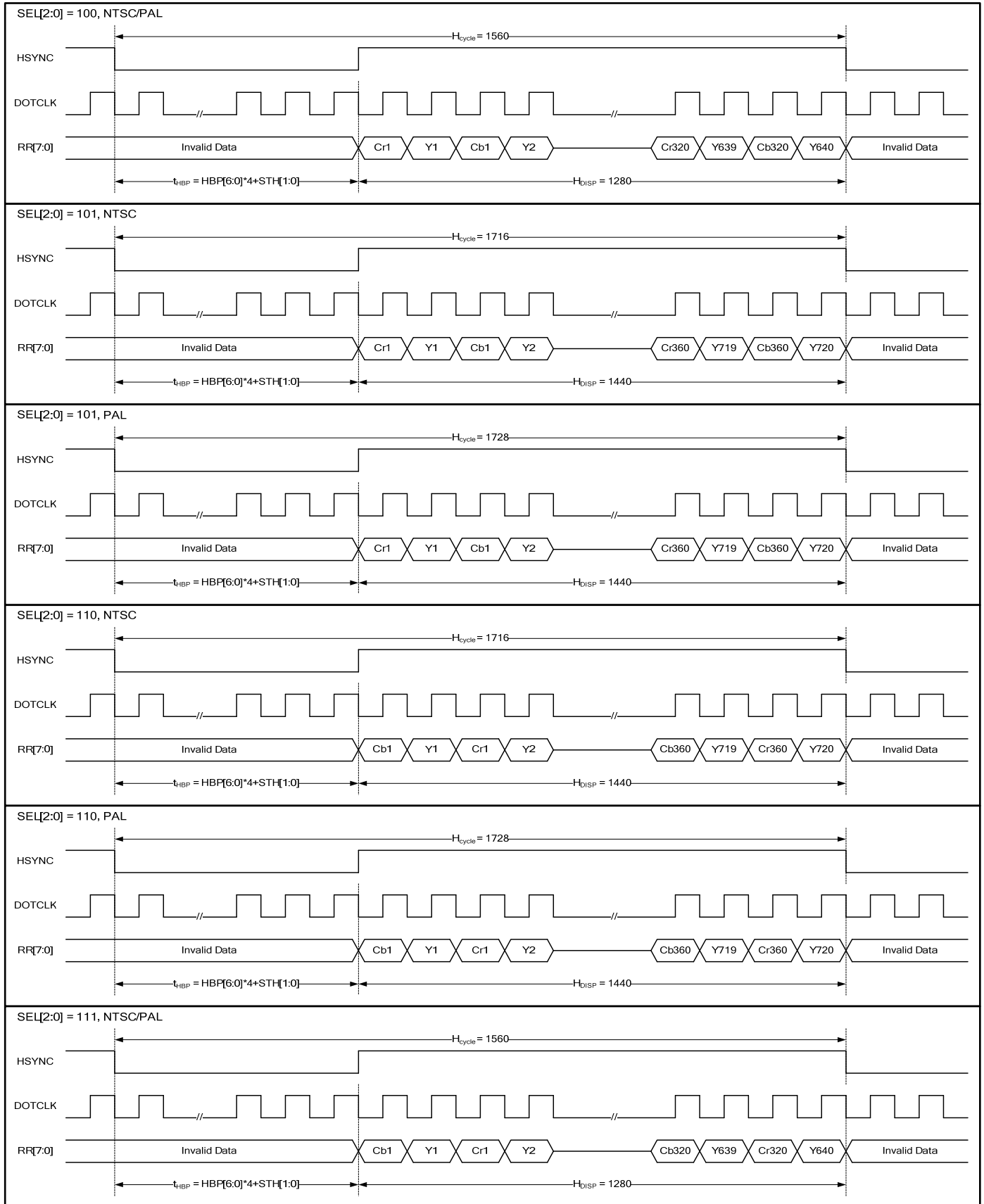
Figure 1 CCIR601 Horizontal Timing
