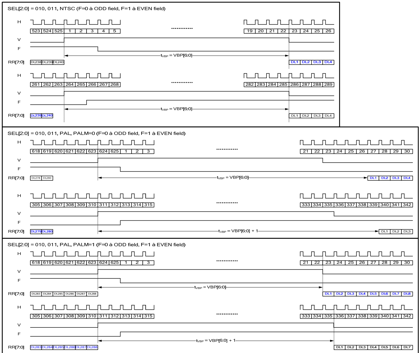
Figure 2 CCIR656 Vertical Timing
