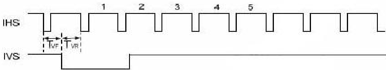
Figure 7 IHS and IVS timing waveforms
