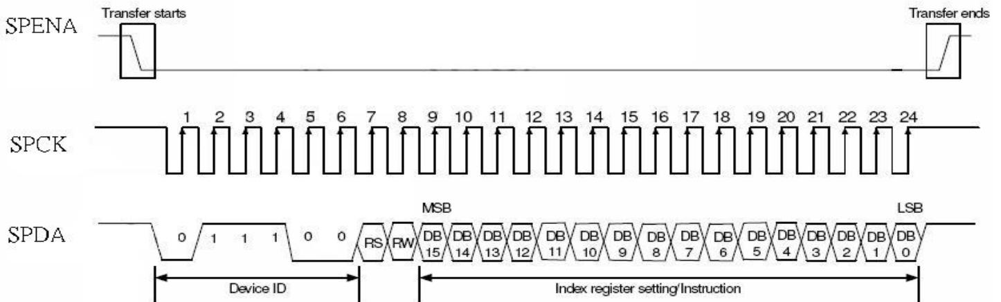
Figure 9 SPI timing
