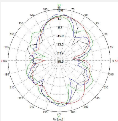
H-Cut ( \theta = 90^\circ )
