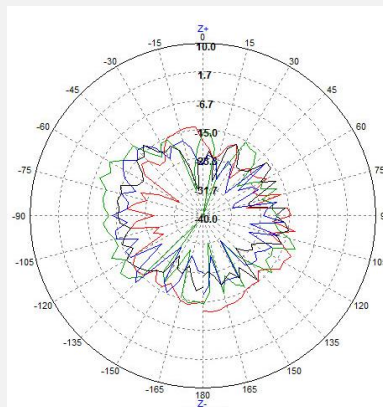
E1-Cut ( \varphi = 0^\circ )
