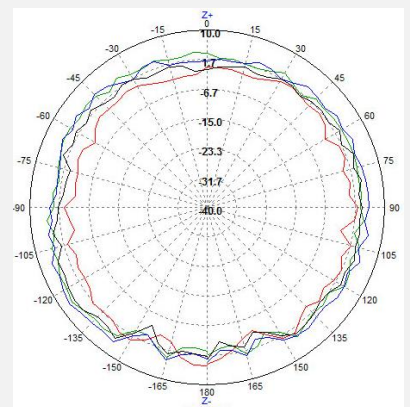
E2-Cut ( \varphi = 90^\circ )
