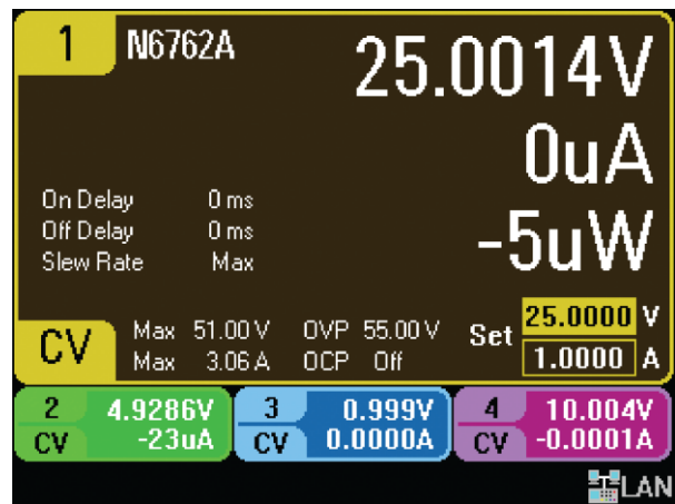
Figure 3. In Meter View, you can also view an enlarged view of one channel, displaying many settings and measured values, for that channel.
