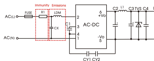
Recommended circuit 2
