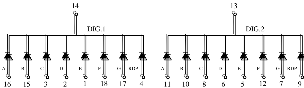
YDSR-2056KM (Common Cathode)
