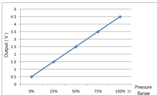
Power Supply:5Vdc
