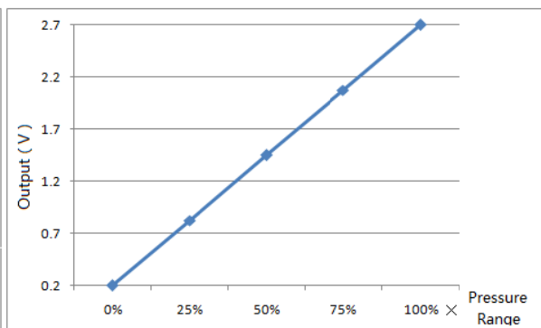
Power Supply:3.3Vdc
